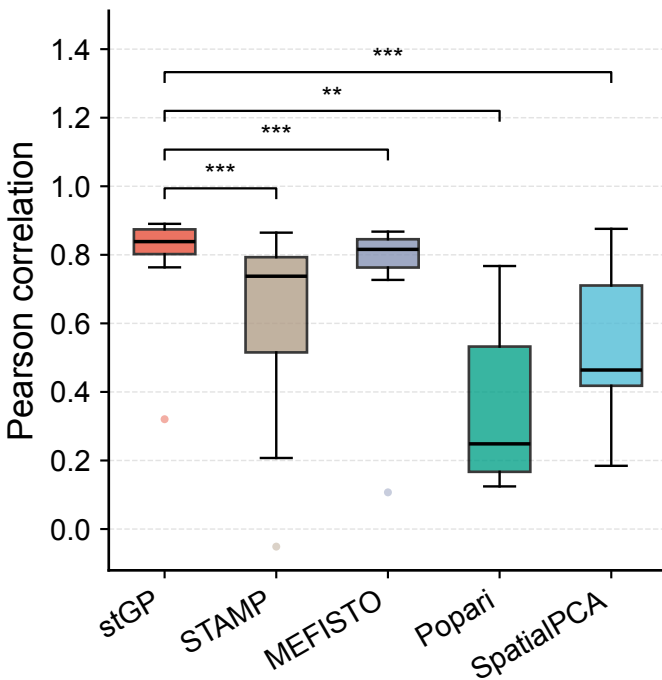
L2/3 ( CUX2 )
