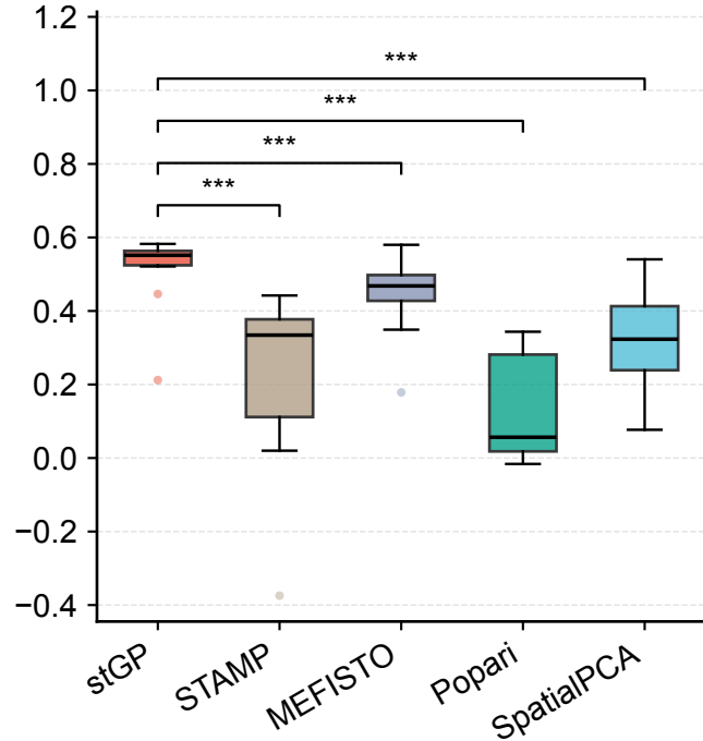
L5/6 ( HS3ST4 )
